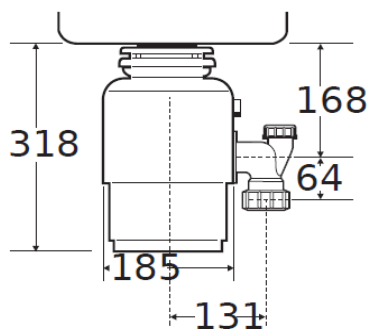
Dimensions (mm)
